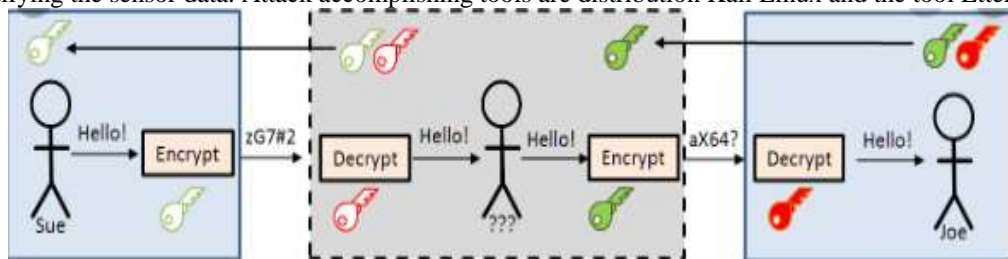
Figure 10 Man-in-the-middle attack in MQTT
