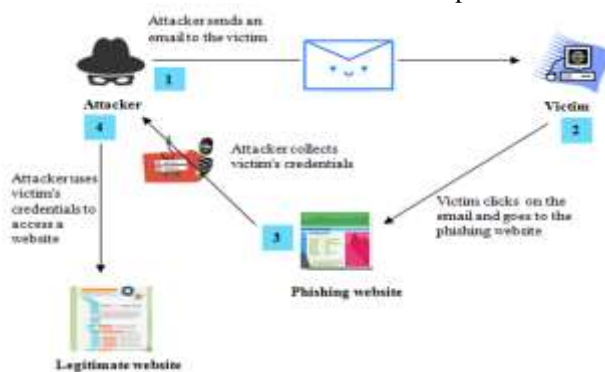
Figure 6. Phishing Attack
