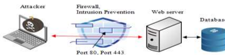
Figure 7. Intrusion Attack
