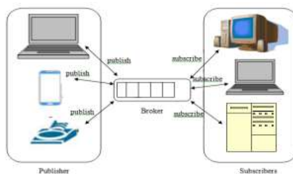
Figure 2. The Architecture of MQTT Protocol
