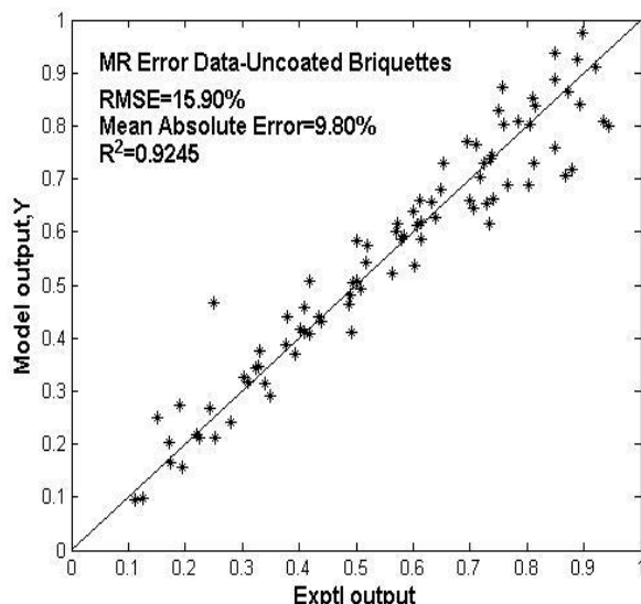
Fig. 1 Multiple regression model out vs. experimental output for uncoated data
